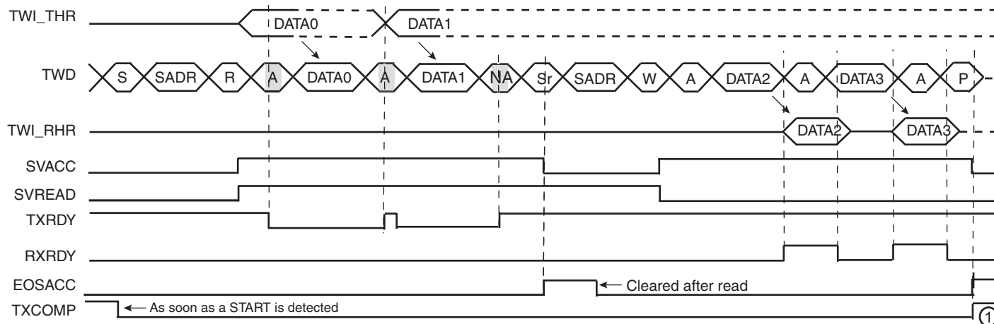
Figure 37-31. Repeated Start + Reversal from Read to Write Mode
