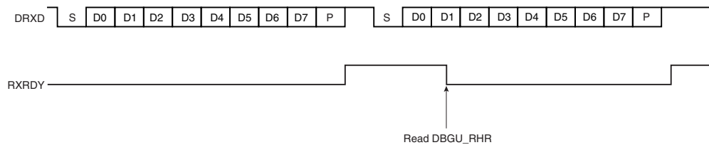
Figure 24-6. Receiver Ready
