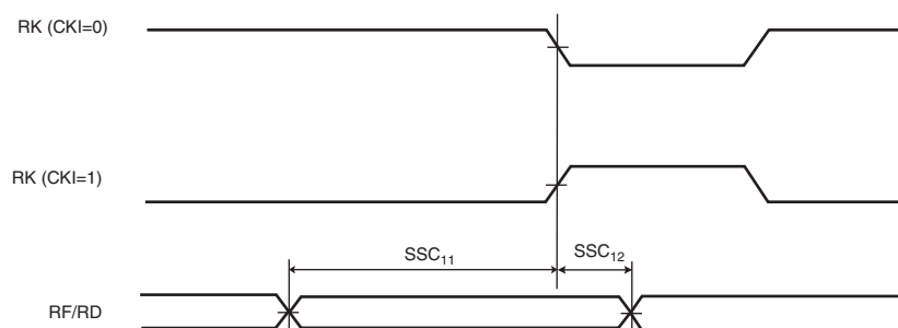
Figure 46-19.SSC Receiver, RK in ouput and RF in input
