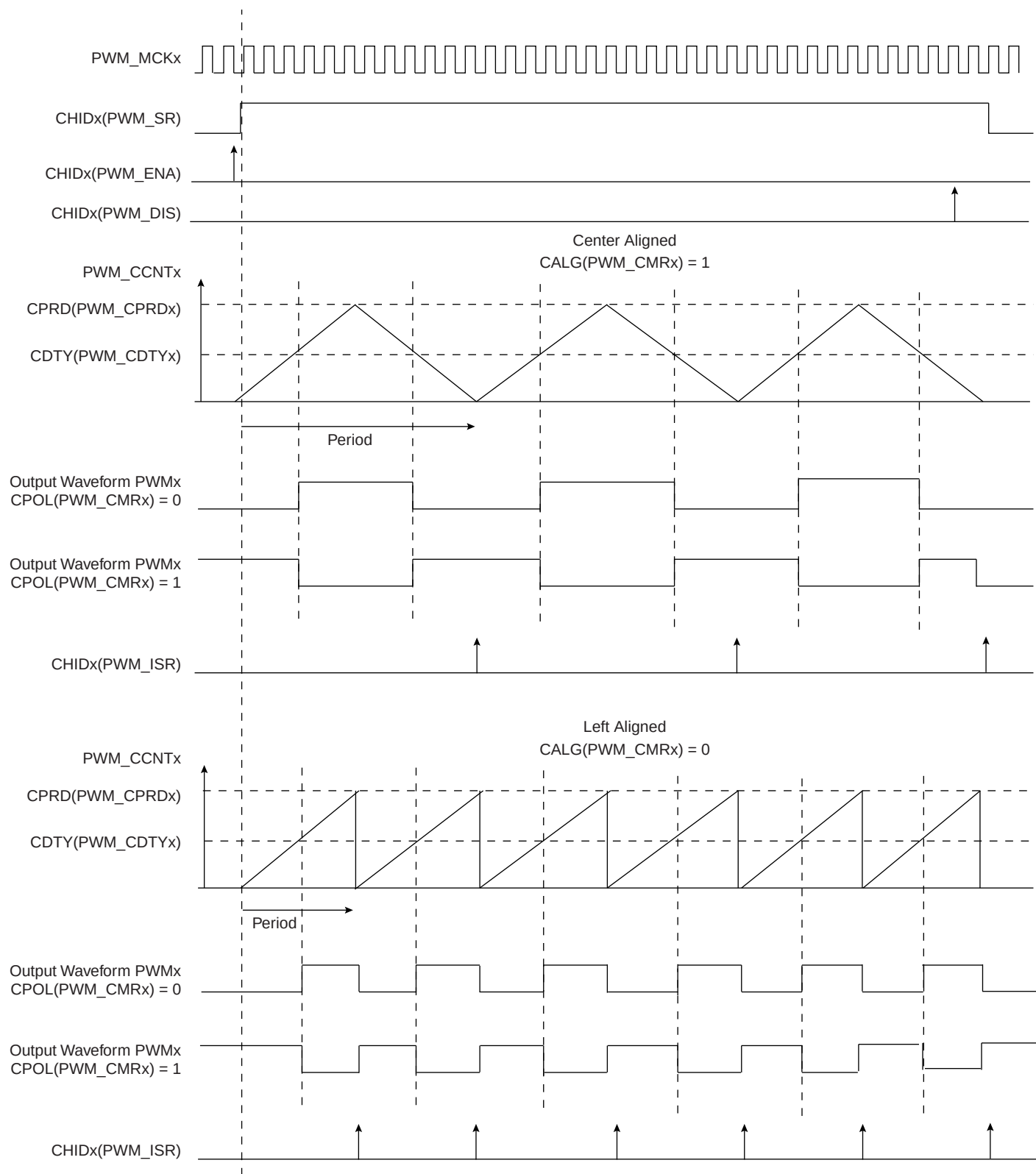
Figure 38-5. Waveform Properties
