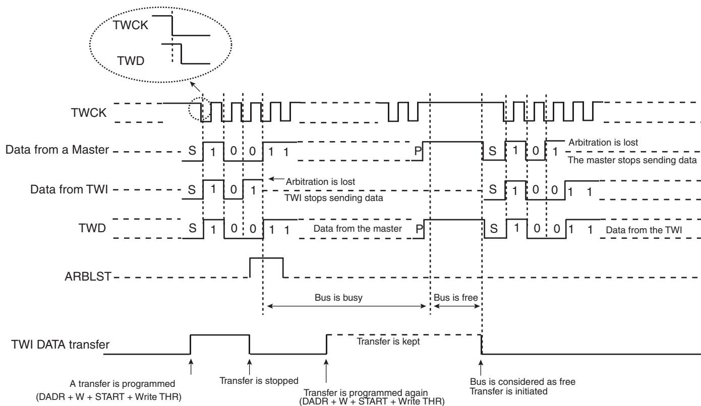
Figure 37-23. Arbitration Cases
