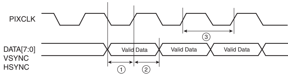
Figure 46-21. ISI Timing Diagram
