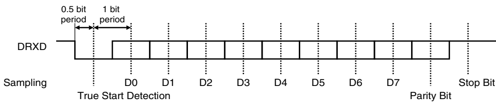
Figure 24-5. Character Reception
