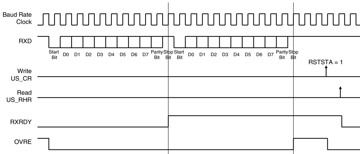
Figure 39-21. Receiver Status
