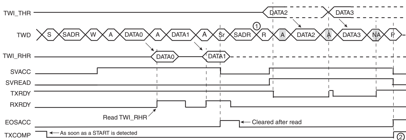
Figure 37-32. Repeated Start + Reversal from Write to Read Mode
