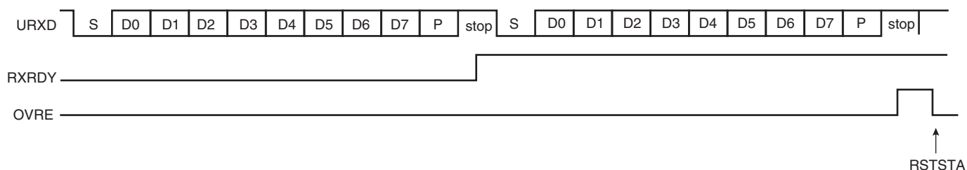
Figure 41-6. Receiver Overrun
