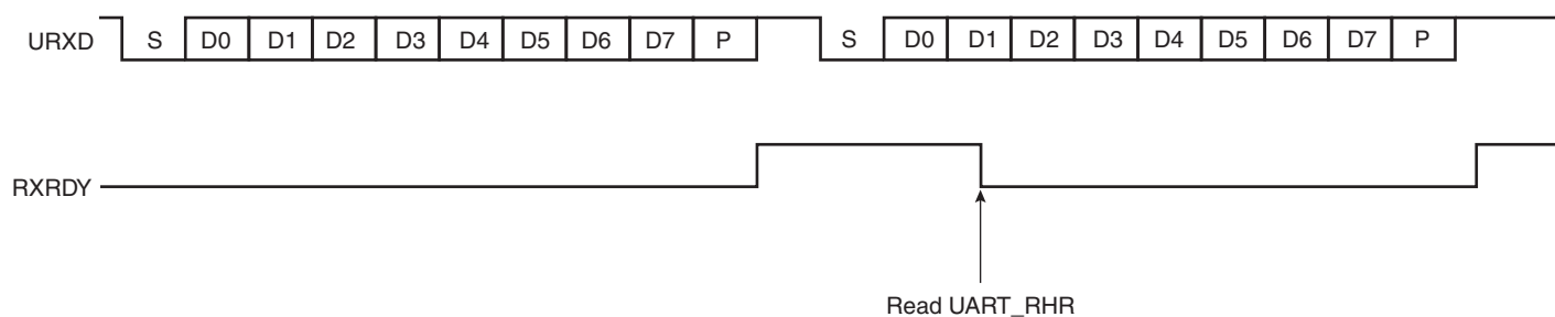
Figure 41-5. Receiver Ready
