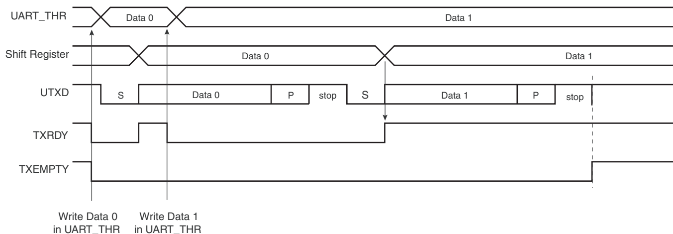
Figure 41-10. Transmitter Control
