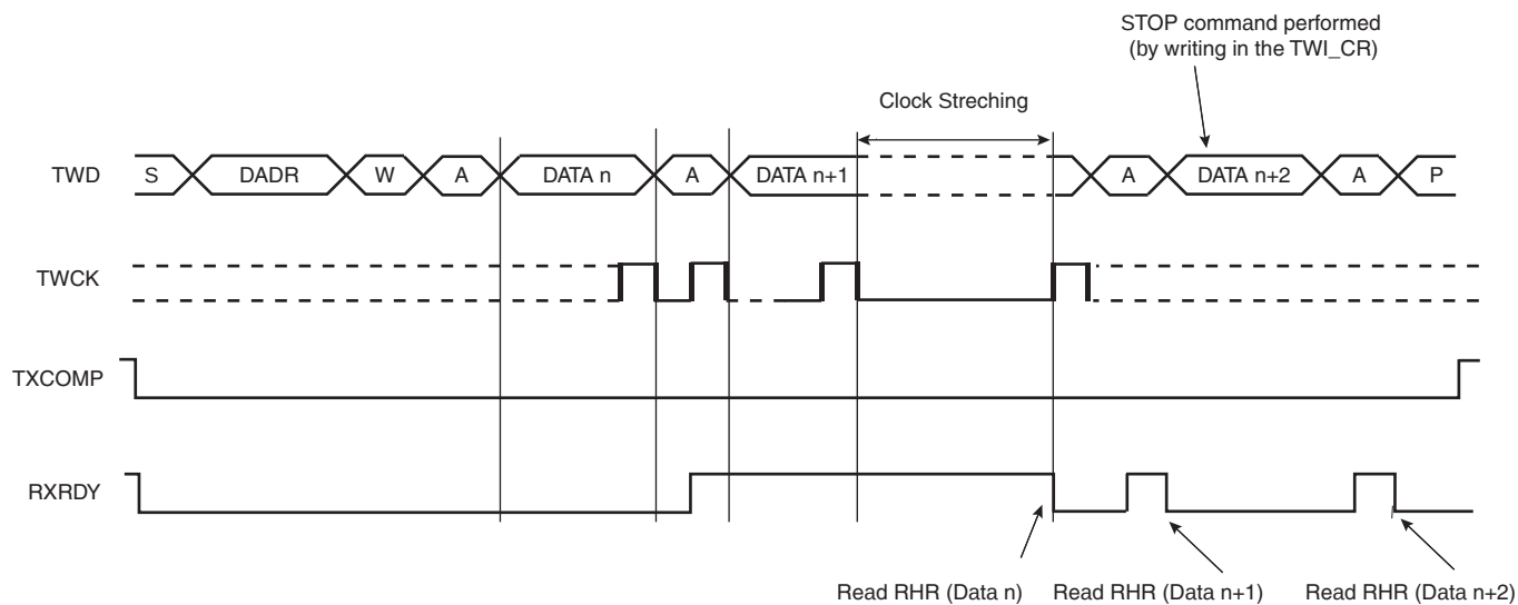
Figure 37-11. Master Read Clock Stretching with Multiple Data Bytes
