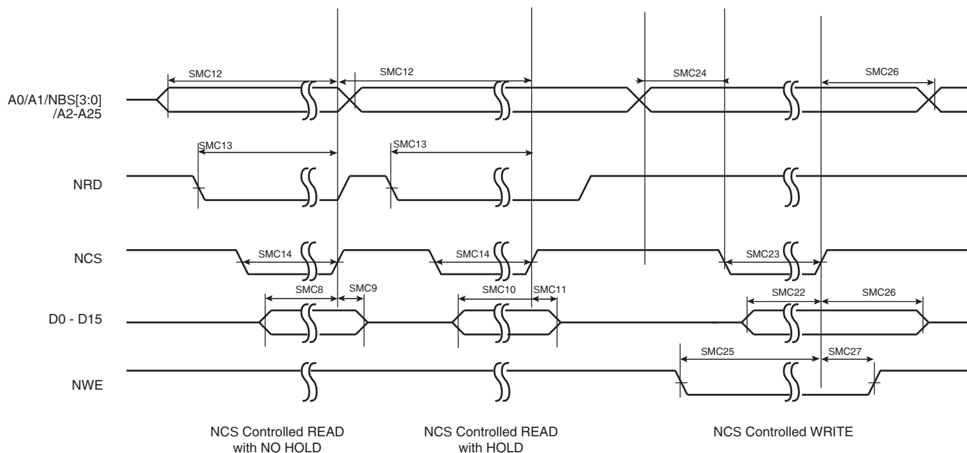
Figure 46-4. SMC Timings - NCS Controlled Read and Write
