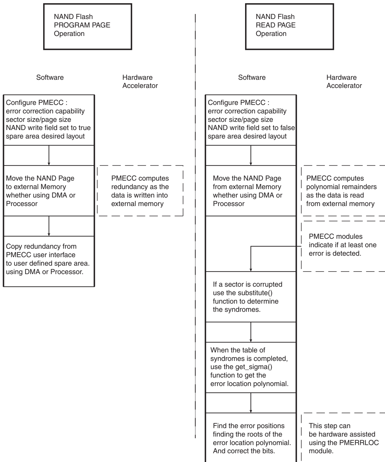
Figure 27-2. Software/Hardware Multibit Error Correction Dataflow
