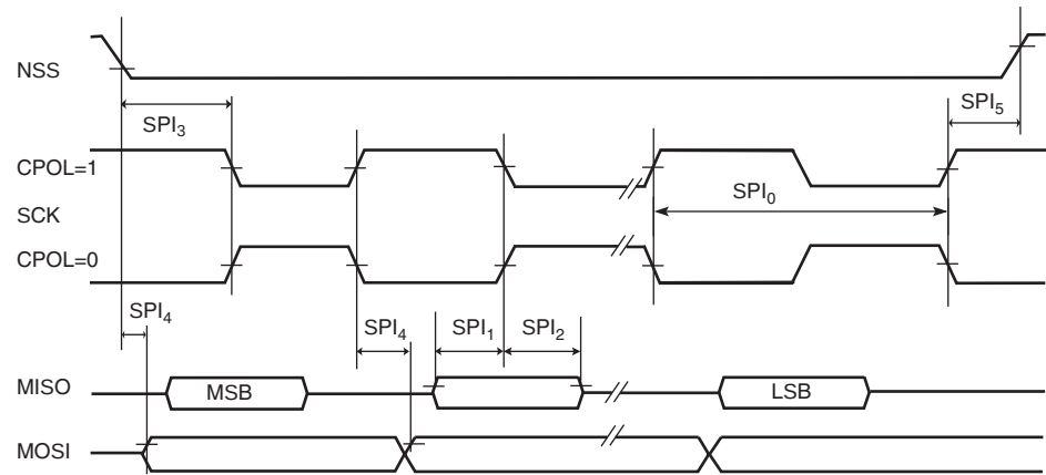
Figure 46-24.USART SPI Master Mode
