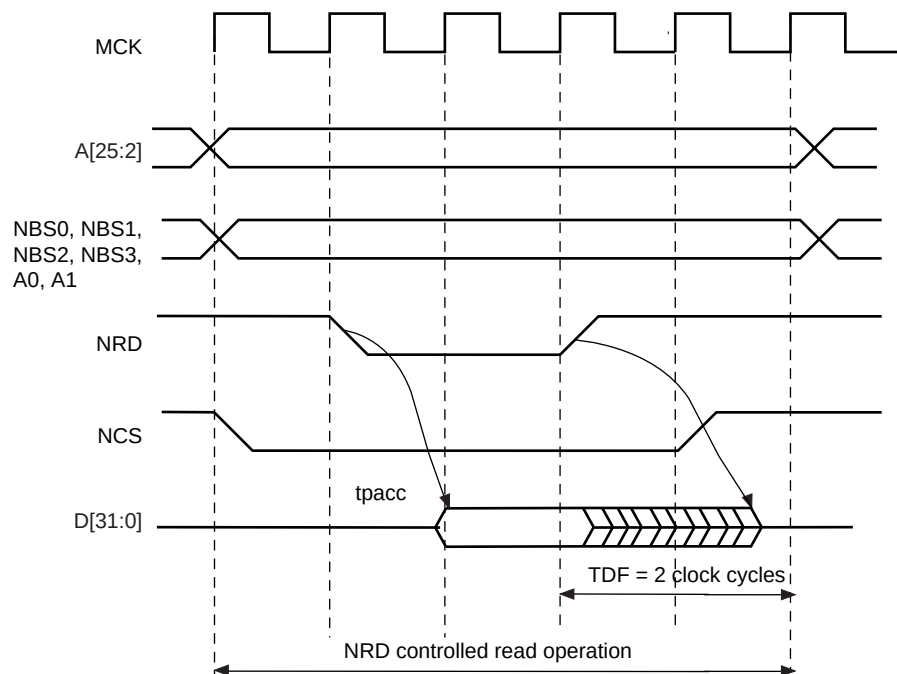
Figure 29-20.TDF Period in NRD Controlled Read Access (TDF = 2)
