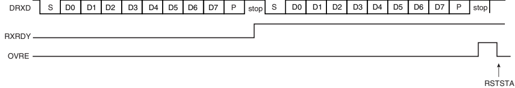
Figure 24-7. Receiver Overrun
