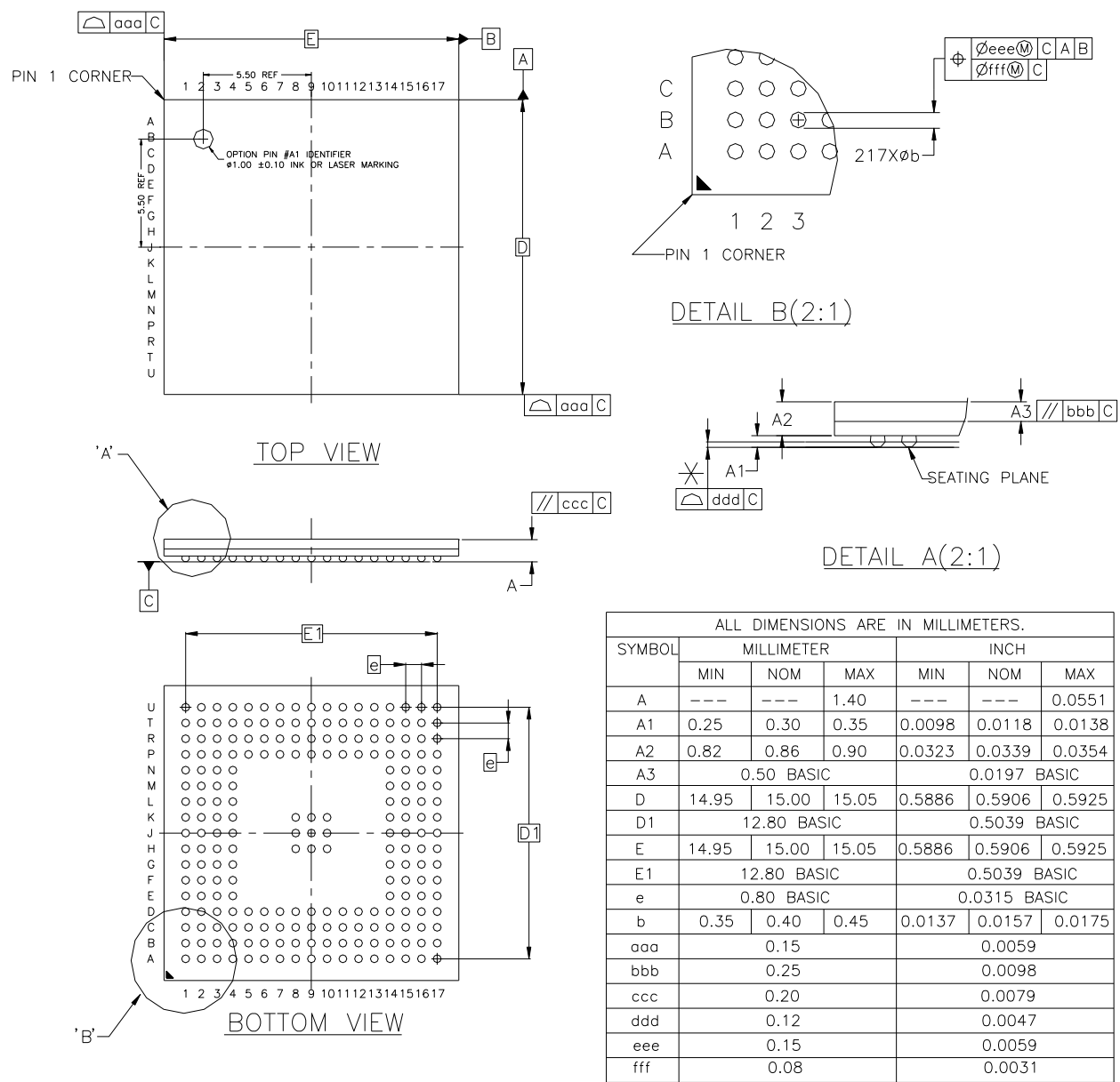
Figure 47-1. 217-ball BGA Package Drawing
