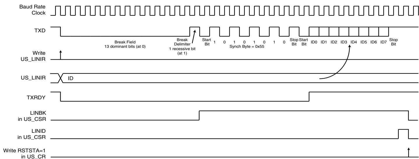
Figure 39-39. Header Transmission
