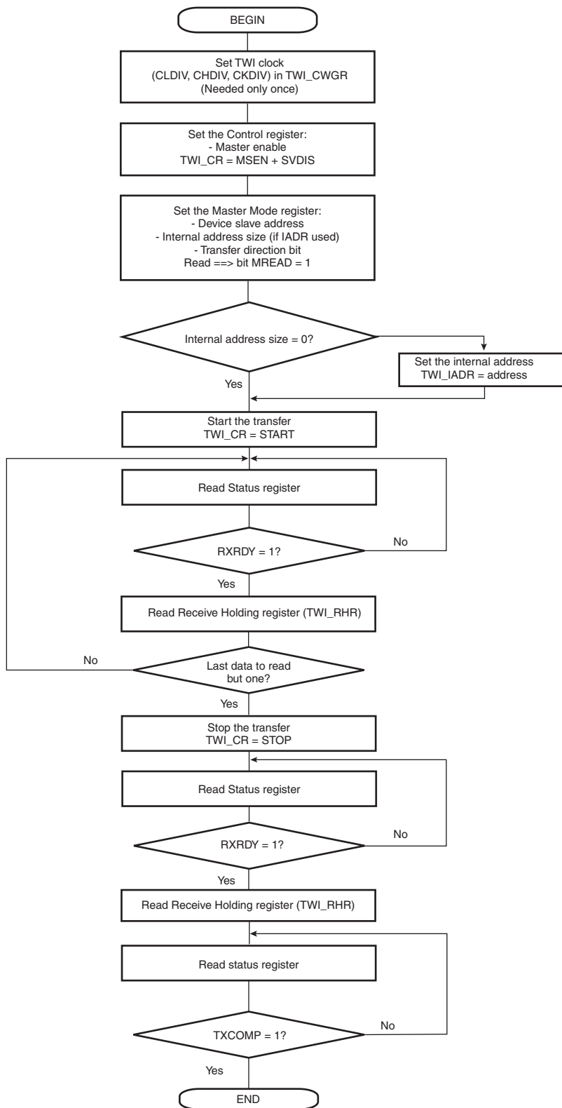
Figure 37-21. TWI Read Operation with Multiple Data Bytes with or without Internal Address
