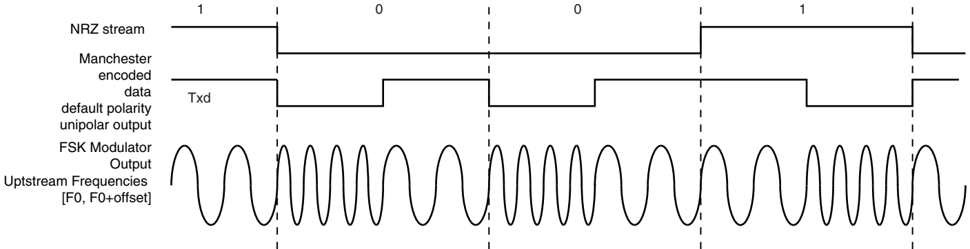
Figure 39-19.FSK Modulator Output
